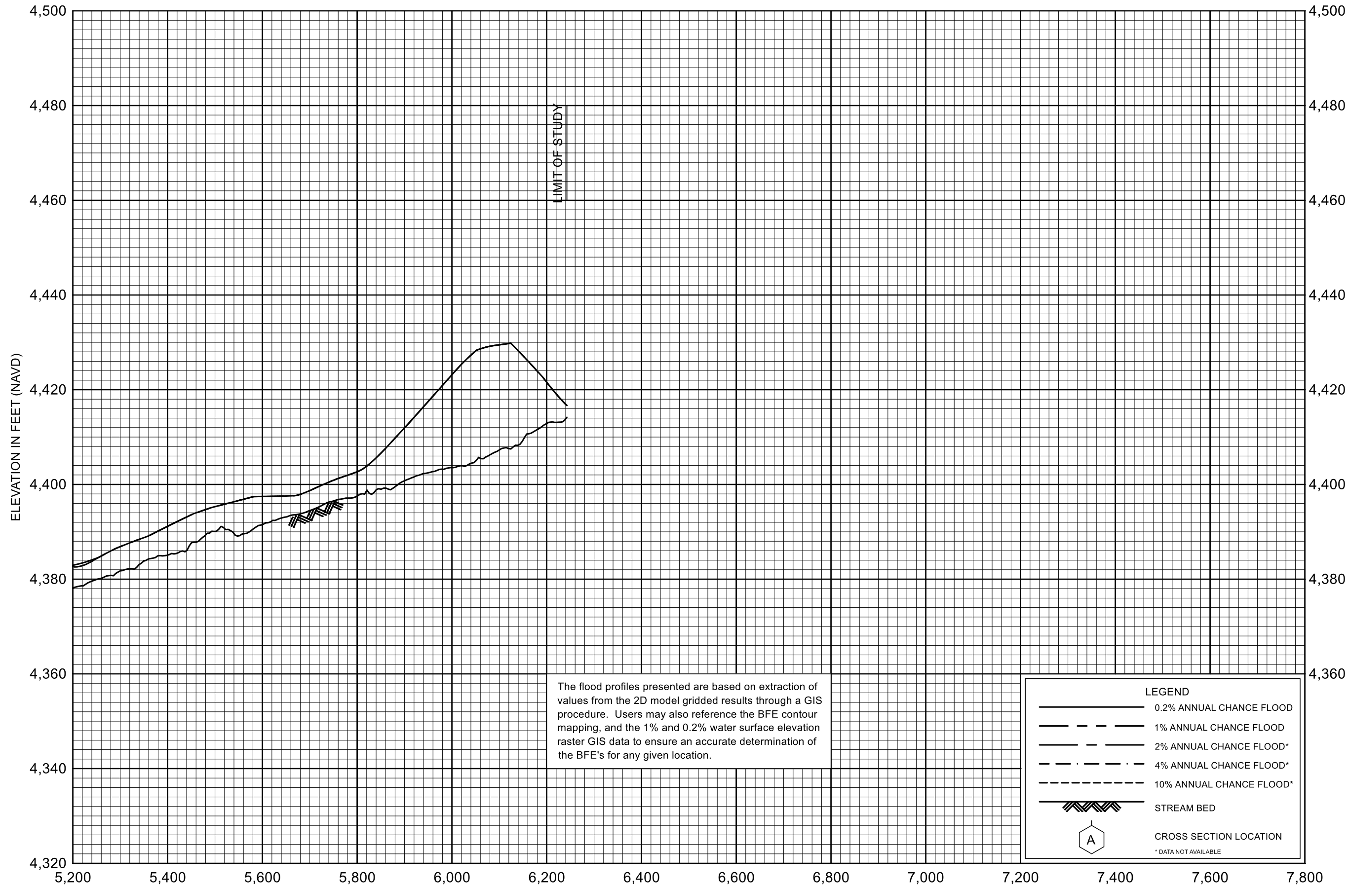
STREAM DISTANCE IN FEET ABOVE DOWNSTREAM LIMIT OF STUDY (APPROX 290 FEET UPSTREAM OF CONFLUENCE WITH FLOW PATH NO. 39A)
